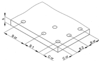
Abb. 1: FHB Highbond-Anker
