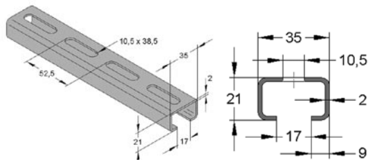
Mefa HST-kisko 35/21/2,00
