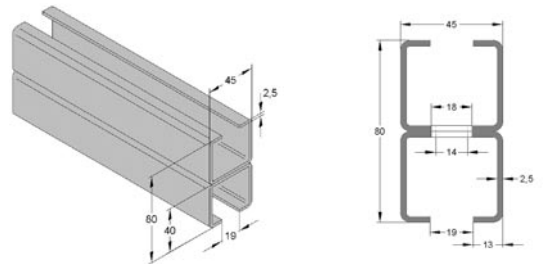
Mefa HST-kisko D 45/80/2,50
