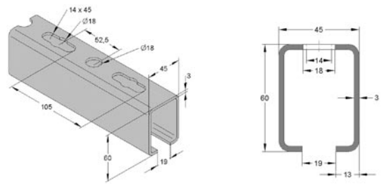
Mefa RST-kisko 45/60/3,00
