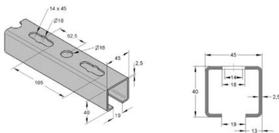
Mefa HST-kisko 45/40/2,50
